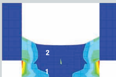
In Windows with rebate bonding and glass edge bonding the IG secondary sealant is in direct contact with the Window adhesive. Therefore, the adhesive must be compatible with the edge sealant. Sika's sealants and adhesive systems are tested and approved to avoid incompatibility. More information about compatibility of our systems can be found on www.sika.com/SES .
