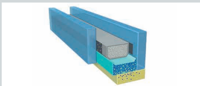
In Windows with rebate bonding and glass edge bonding the IG secondary sealant is in direct contact with the Window adhesive. Therefore, the adhesive must be compatible with the edge sealant. Sika's sealants and adhesive systems are tested and approved to avoid incompatibility. More information about compatibility of our systems can be found on www.sika.com/SES .
